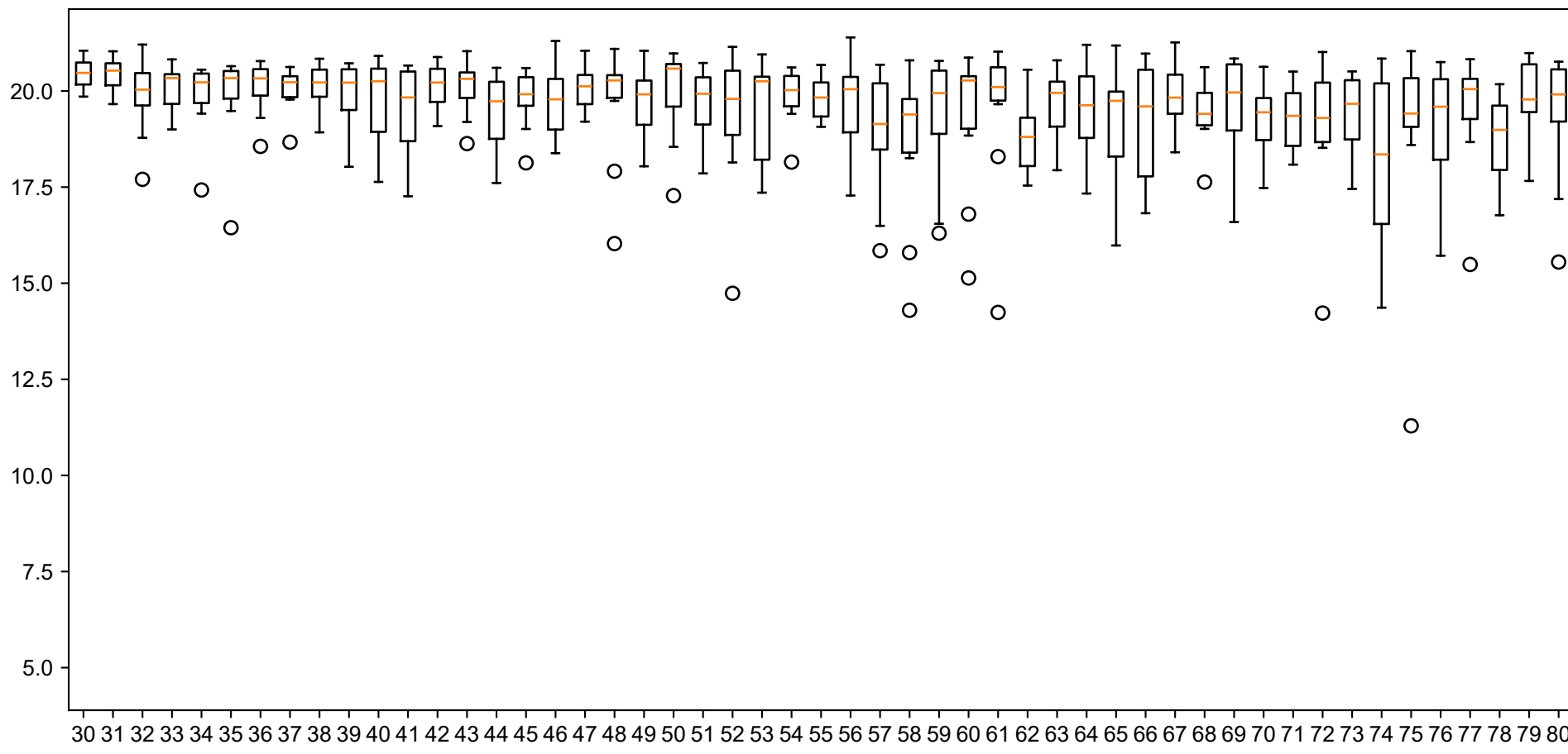
mutual_info_classif
