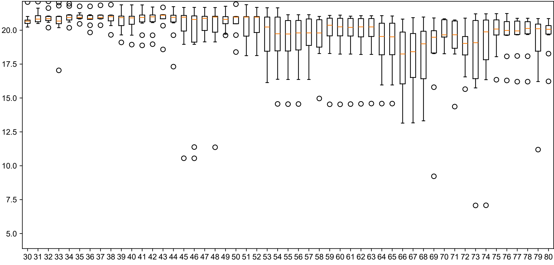
rf
