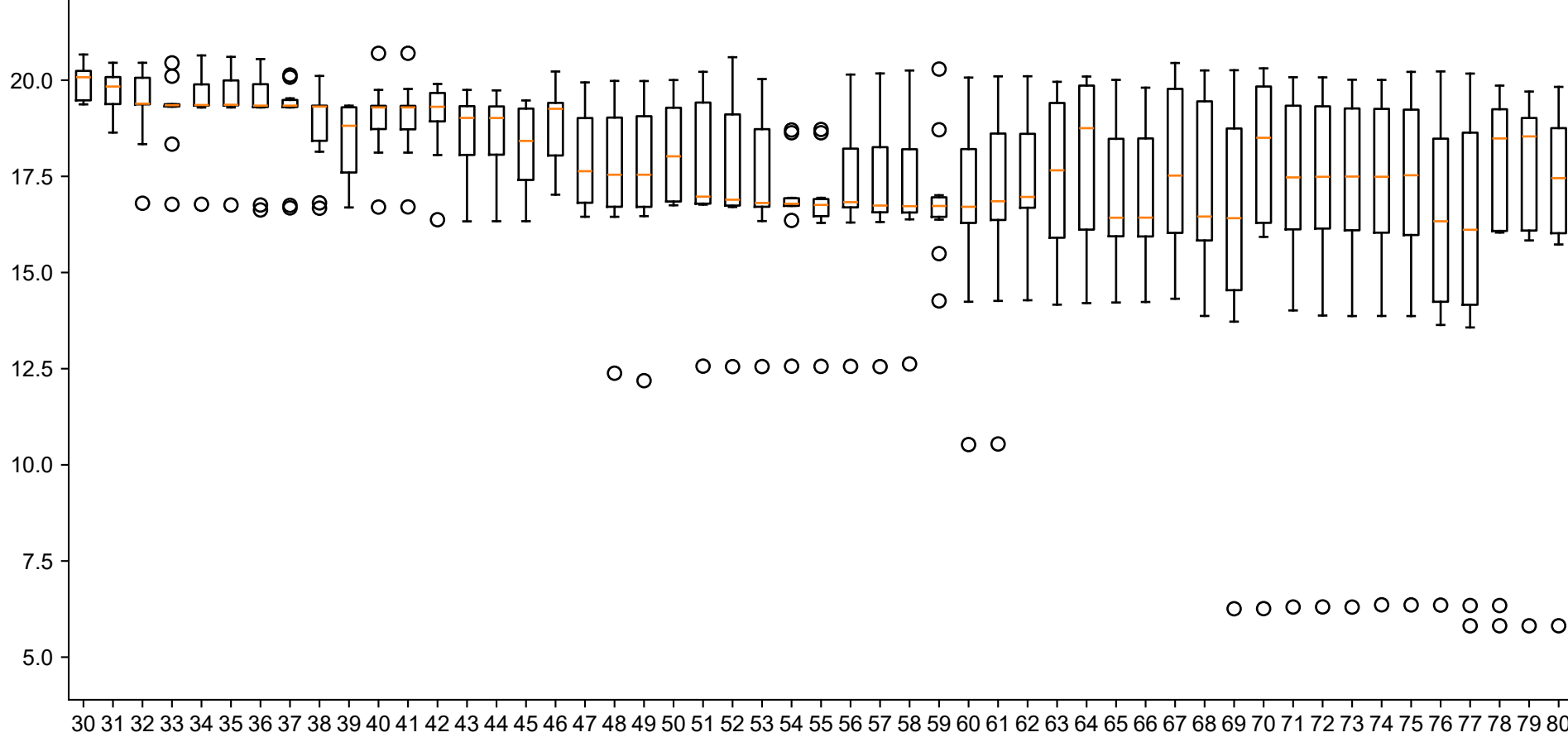
xgb
