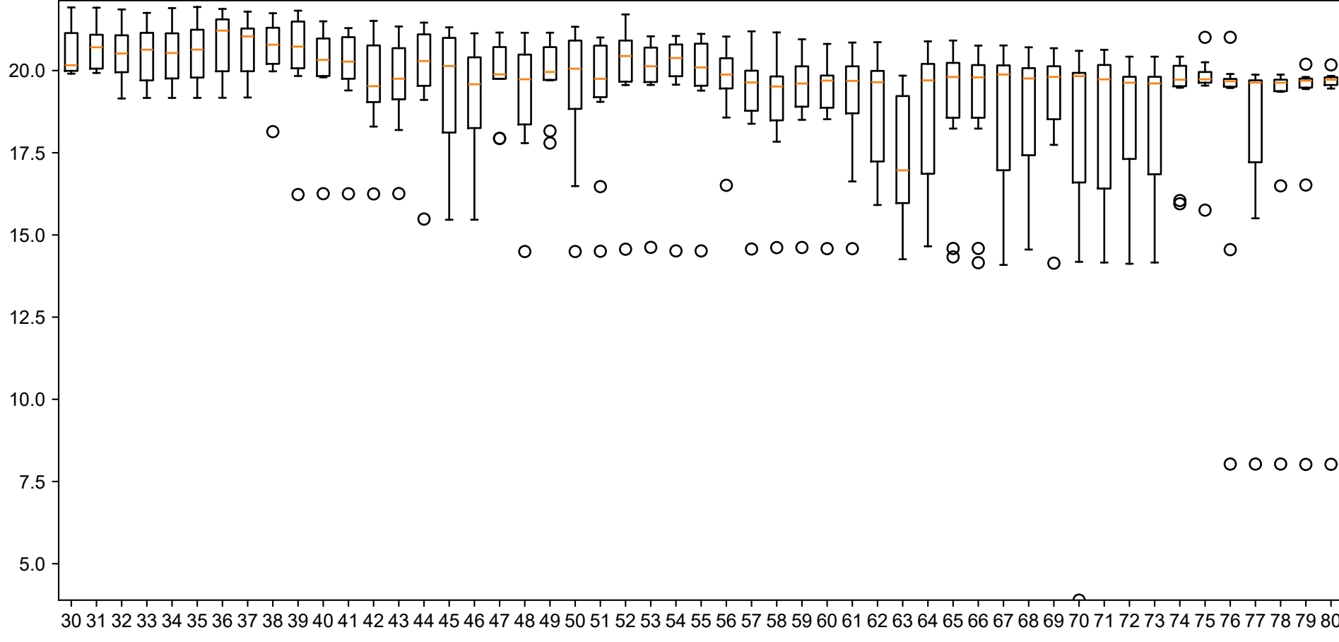
xgb
